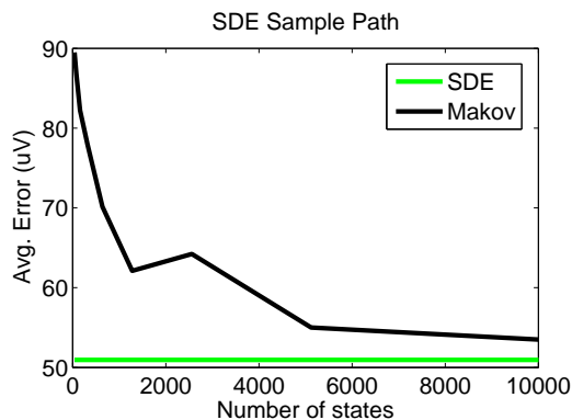
Fig. 13. Average error obtained using Markov models of different number of states compared with SDE
