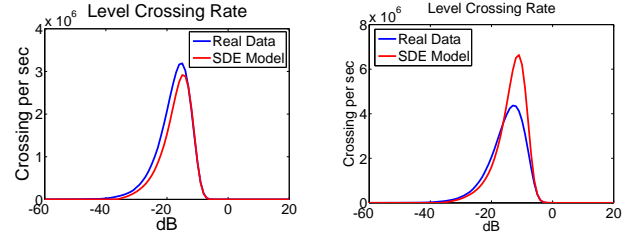
Fig. 6. Level crossing rate of synthesized SDE and measurement data (551MHz left, 629MHz right)
