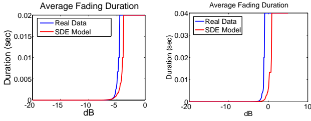
Fig. 7. Average fading duration of synthesized SDE and measurement data (551MHz left, 629MHz right)
