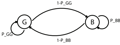
Fig. 8. The Gilbert-Elliott (2-state) model
