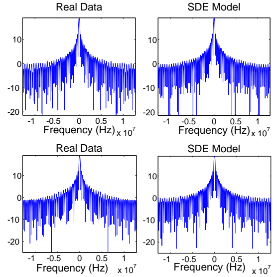
Fig. 5. Power spectral density of synthesized SDE and measurement data (551MHz top, 629MHz bottom)
