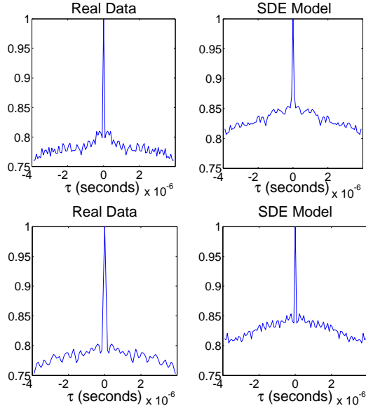
Fig. 4. Autocorrelation of synthesized SDE and measurement data (551MHz top, 629MHz bottom)
