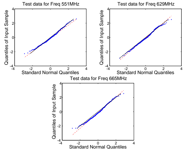
Fig. 1. Q-Q plot, 551MHz (top left), 629MHz (top right), 665MHz (bottom)
