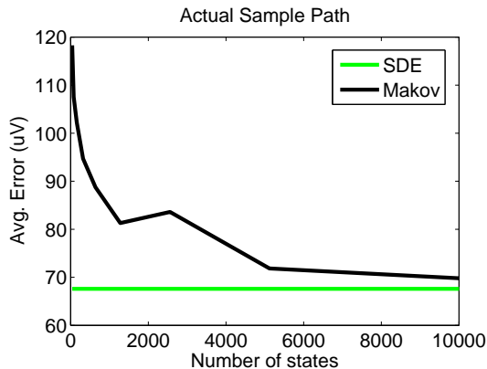
Fig. 12. Average error obtained using Markov models of different number of states compared with SDE
