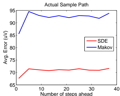
Fig. 14. Average error obtained using a 1000-state Markov model and SDE for n -step prediction.
