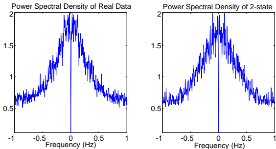
Fig. 10. The power spectral density of real data and the GE model over a 300-second duration.
