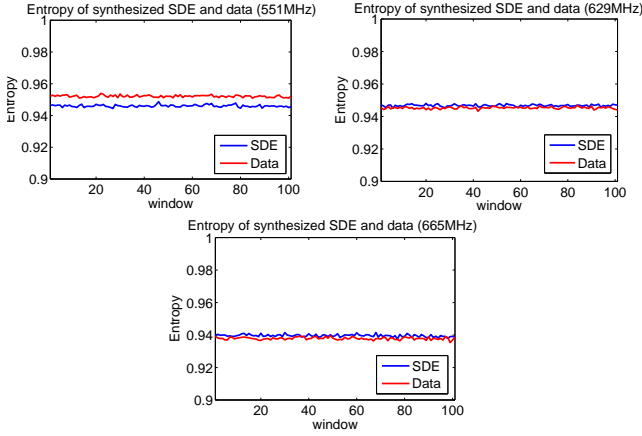
Fig. 3. Entropy of synthesized SDE and data (551MHz top left, 629MHz top right, 665MHz bottom)
